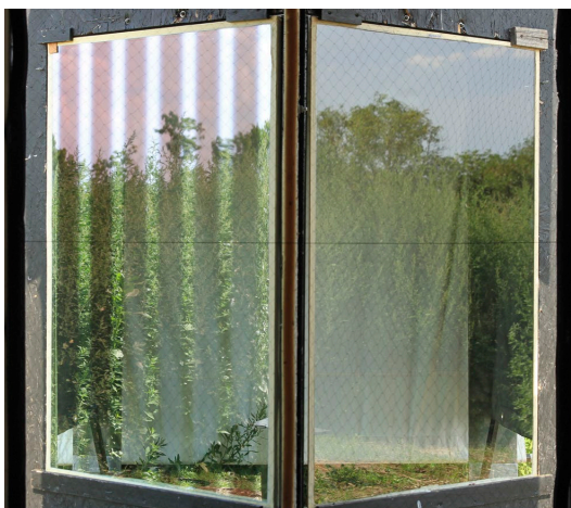
Bird's-eye view in the test tunnel. Pilkington AviSafe™ exterior view: highly effective as protection against bird collision, barely visible from the interior (left: test pane, right: reference pane).
