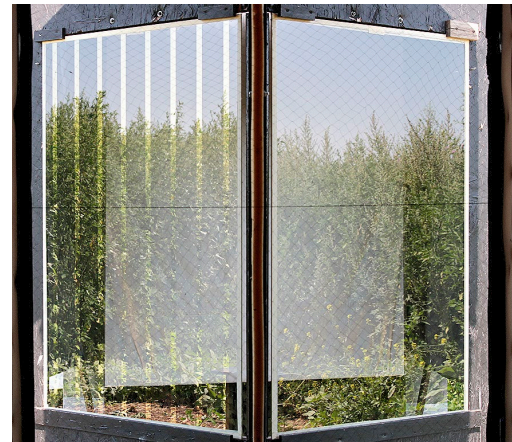
A marking currently being developed by the Fraunhofer Institute for Solar Energy Systems (ISE), with transparent stripes on surface 1, proved to be highly effective (left: test pane, right: reference pane).
